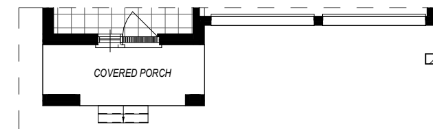
MAIN FLOOR PLAN ELEV. C 1460 SQ.FT
