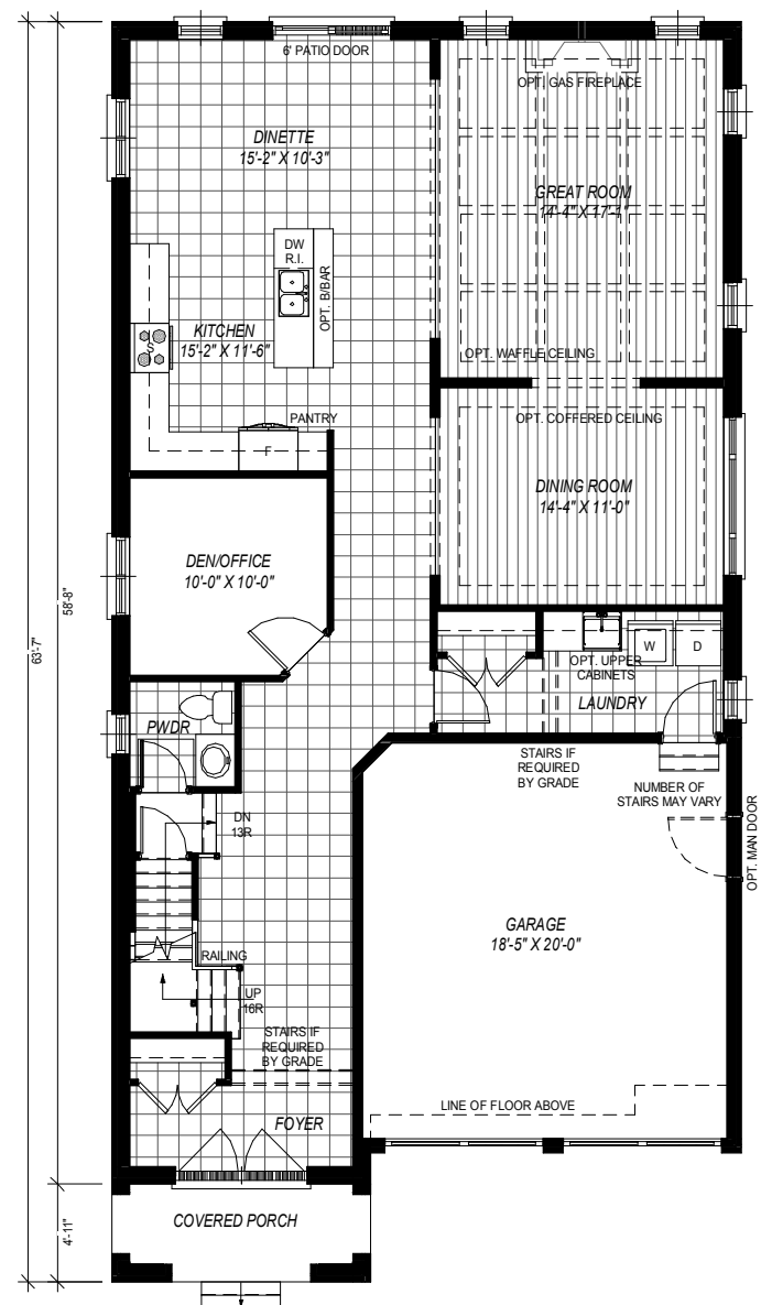
MAIN FLOOR PLAN 1460 SQ.FT
