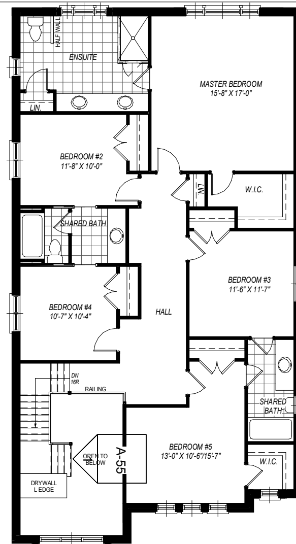
ALT. SECOND FLOOR PLAN 5 BED 1817 SQ.FT (INCLUDES 138 SF OTB)
