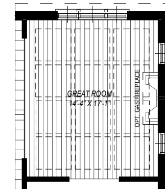
ALT. MAIN FLOOR PLAN 1460 SQ.FT
