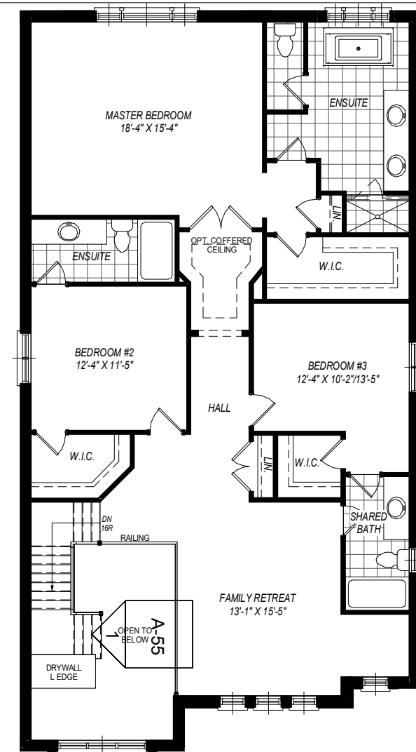
ALT. SECOND FLOOR PLAN FAMILY RETREAT 1817 SQ.FT (INCLUDES 138 SF OTB)
