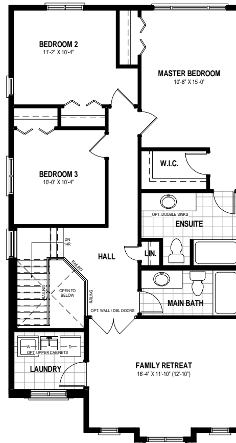
SECOND FLOOR PLAN 1159 SQ. FT.
