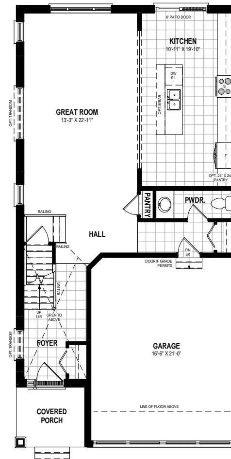
MAIN FLOOR PLAN ALT 1 867 SQ. FT.
