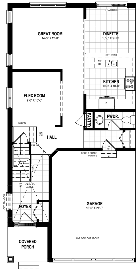
MAIN FLOOR PLAN 867 SQ. FT.
