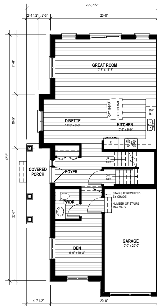
MAIN FLOOR PLAN 839 SQ. FT.
