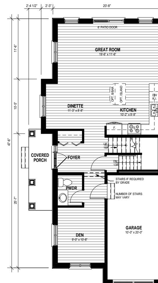
ALT. FLOOR LAYOUT EASY LIVING 839 SF. FT.
