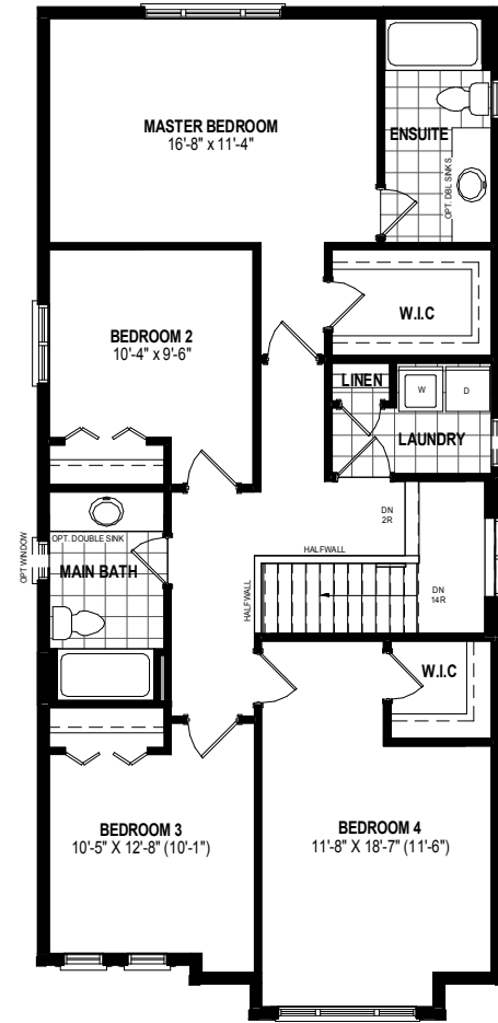
SECOND FLOOR PLAN ALT 2 1206 SQ. FT.
