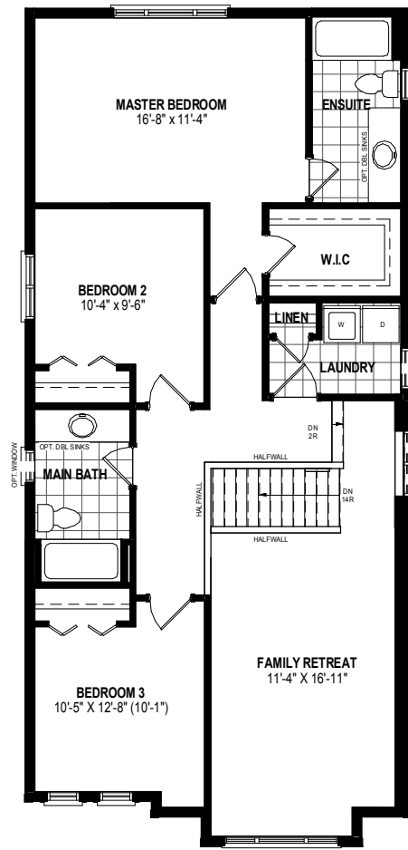
SECOND FLOOR PLAN ALT 1 1206 SQ. FT.
