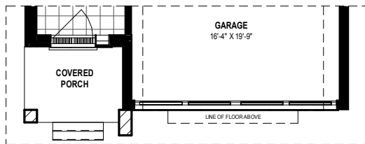
PARTIAL FLOOR PLAN ELEVATION 'C' 918 SQ. FT.
