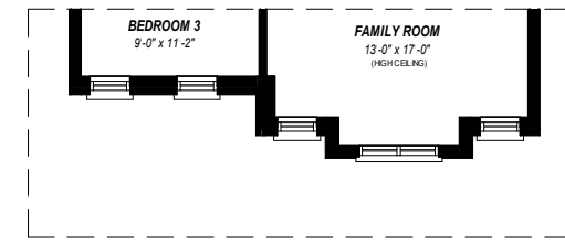
PARTIAL ELEVATION 'B' 1196 SQ.FT
