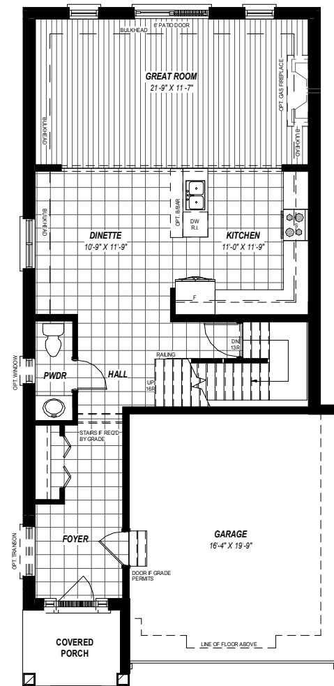
MAIN FLOOR PLAN ALT 1 918 SQ.FT
