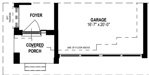
PARTIAL MAIN FLOOR PLAN ELV 'C' 919 SQ. FT.
