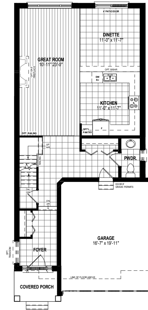
MAIN FLOOR PLAN. ALT 2 919 SQ. FT.
