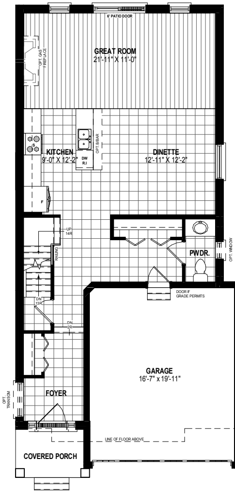
MAIN FLOOR PLAN 919 SQ. FT.
