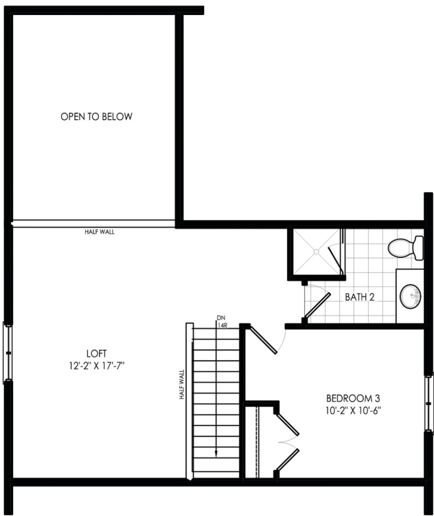
OPT. LOFT Floor Area: 556 s.f.
