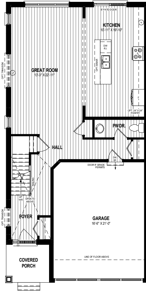
MAIN FLOOR PLAN ALT 1 872 SQ. FT.
