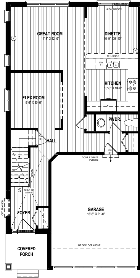
MAIN FLOOR PLAN ALT 2 872 SQ. FT.
