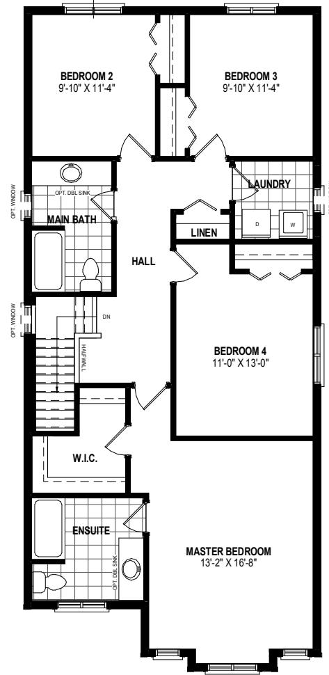
SECOND FLOOR PLAN ALT 1 1221 SQ.FT
