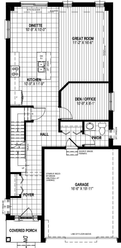
MAIN FLOOR PLAN 914 SQ.FT
