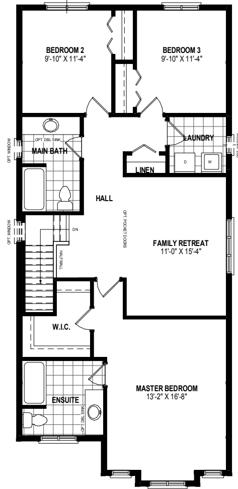
SECOND FLOOR PLAN 1221 SQ.FT
