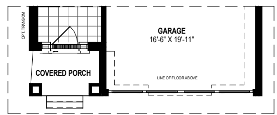
PARTIAL MAIN FLOOR ELV 'B' 914 SQ.FT
