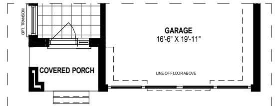
PARTIAL MAIN FLOOR ELV 'C' 914 SQ.FT
