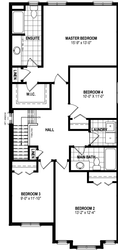
SECOND FLOOR PLAN ALT 2 1221 SQ.FT
