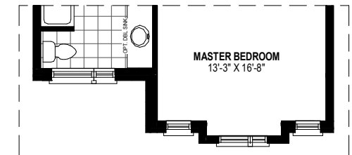
PARTIAL SECOND FLOOR PLAN ELV 'C' 1221 SQ.FT
