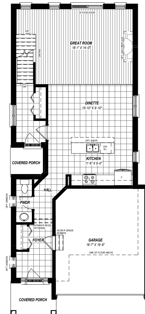
MAIN FLOOR PLAN 951 SQ.FT (ELEVATION A SHOWN)
