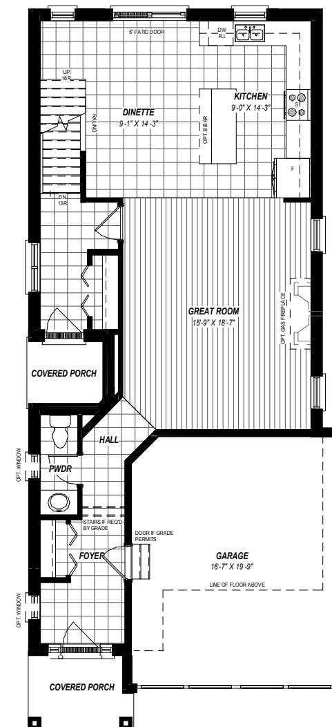
MAIN FLOOR PLAN ALT 1 951 SQ.FT (ELEVATION B SHOWN)
