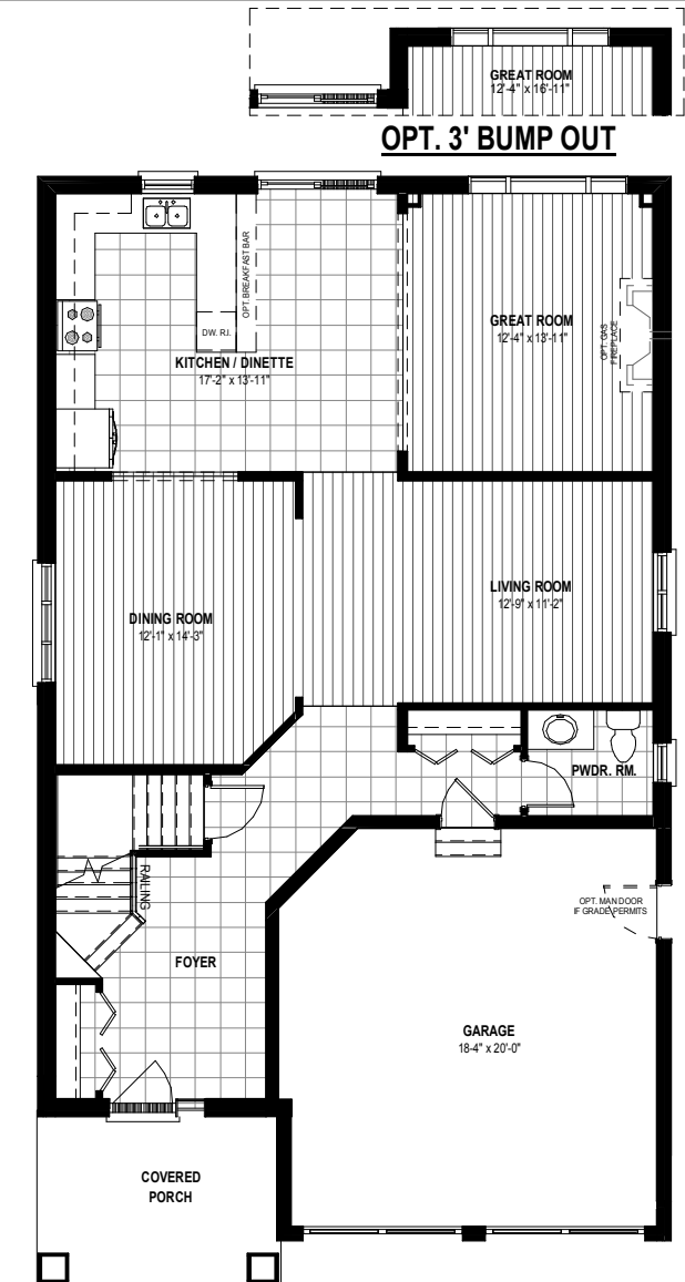
MAIN FLOOR PLAN ALT 2 1,245 SQ.FT (1287 W/ BUMP OUT) (ELEVATION A SHOWN)
