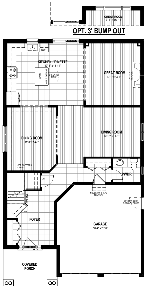
MAIN FLOOR PLAN 1,245 SQ.FT (1287 W/ BUMP OUT) (ELEVATION A SHOWN)
