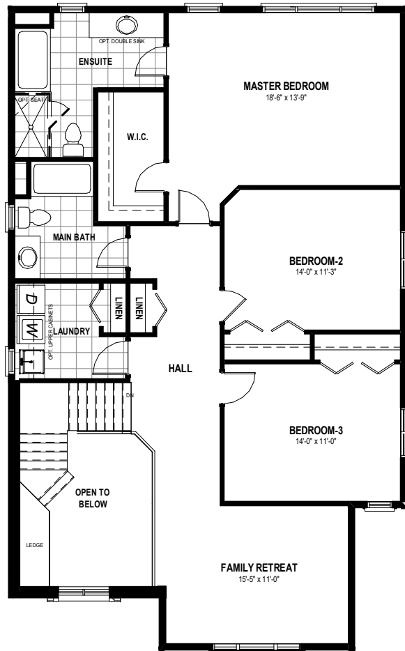
SECOND FLOOR PLAN 1,561 SQ.FT. (INCL. 108 SQ. FT. O.T.B.) (ELEVATION A SHOWN)
