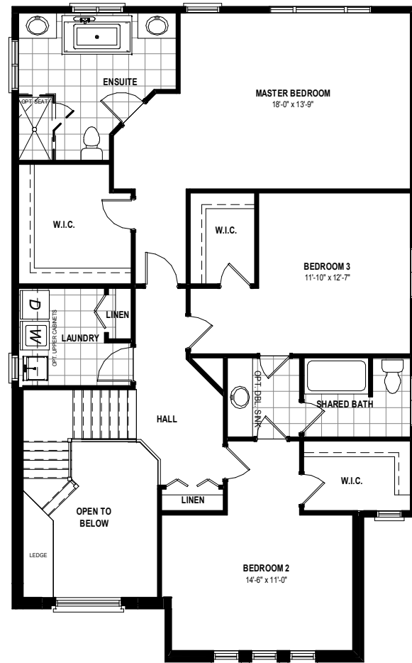
MAIN FLOOR PLAN ALT 1 1,561 SQ.FT. (INCL. 108 SQ. FT. O.T.B.) (ELEVATION B SHOWN)
