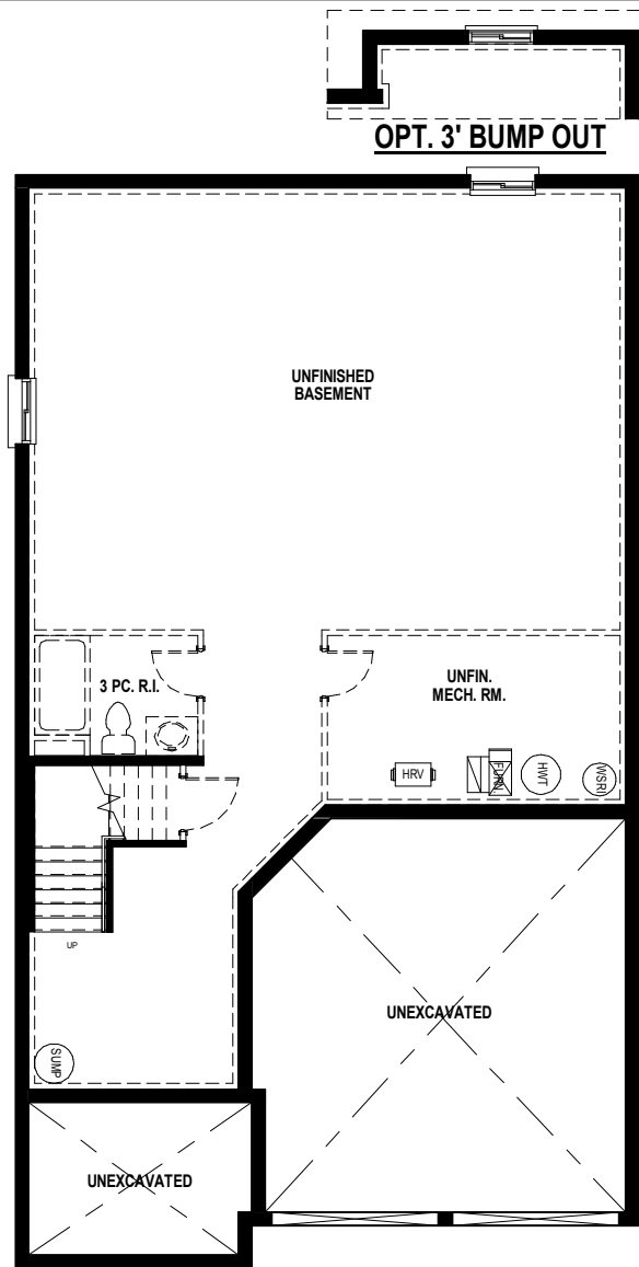
BASEMENT PLAN STANDARD
