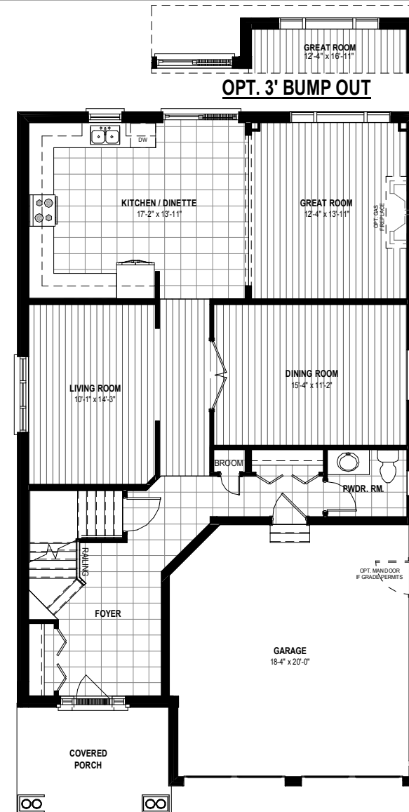
MAIN FLOOR PLAN ALT 1 1,245 SQ.FT (1287 W/ BUMP OUT) (ELEVATION A SHOWN)
