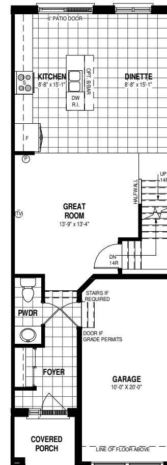
MAIN FLOOR PLAN ALT. 1 665 SQ.FT (680 SQ. FT. END UNIT) 18' ~ MIDTOWN SERIES
