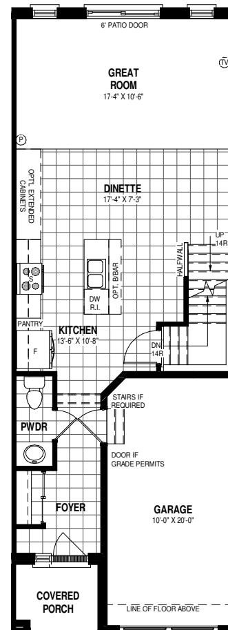
MAIN FLOOR PLAN 665 SQ.FT (680 SQ. FT. END UNIT)
