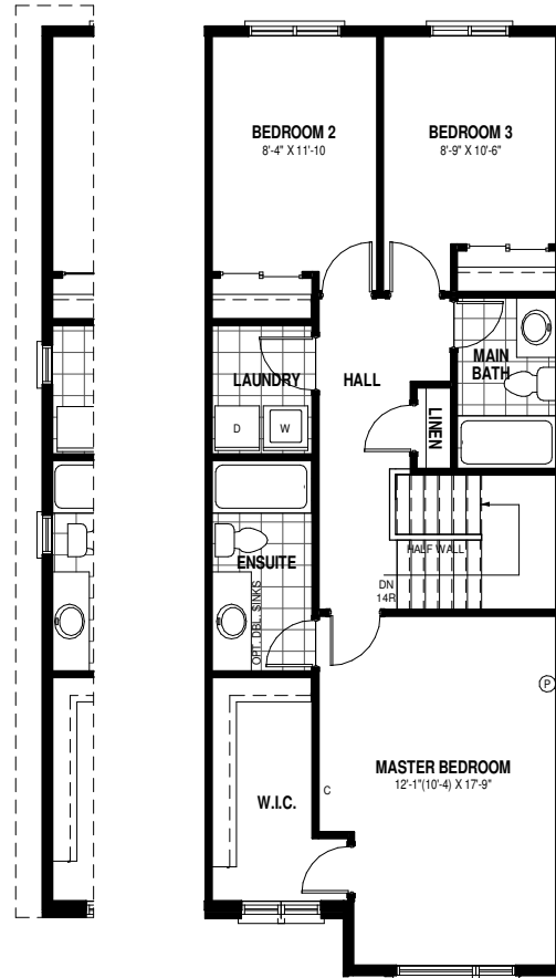
SECOND FLOOR PLAN 853 SQ.FT (869 SQ. FT. END UNIT)
