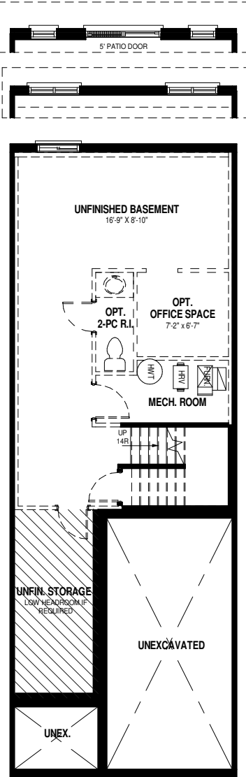
BASEMENT FLOOR PLAN
