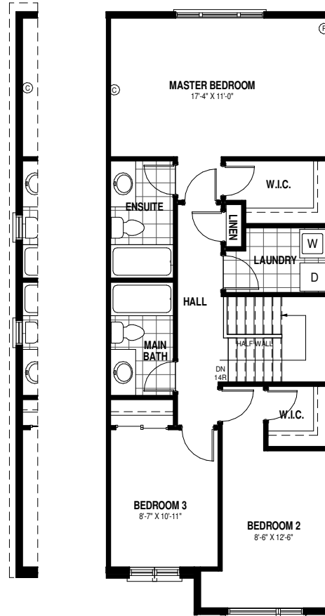
SECOND FLOOR PLAN ALT. 1 853 SQ.FT (869 SQ. FT. END UNIT)
