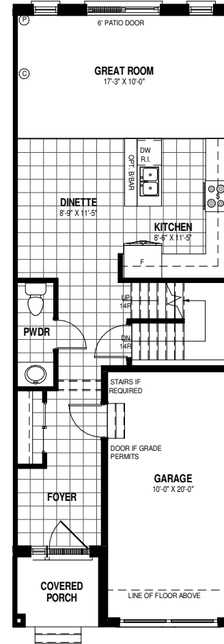
MAIN FLOOR PLAN ALT. 1 665 SQ.FT (680 SQ. FT. END UNIT)
