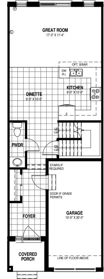
MAIN FLOOR PLAN ALT. 2 665 SQ.FT (680 SQ. FT. END UNIT)
