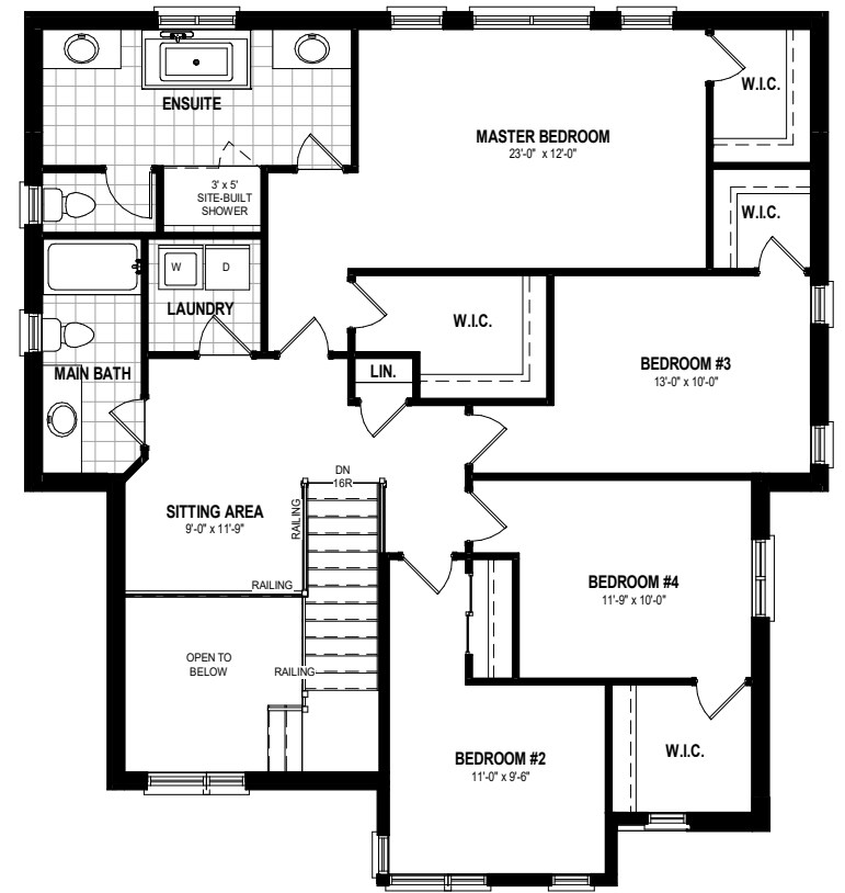
SECOND FLOOR PLAN 1,570 SQ.FT (INCL. 75 OTB)
