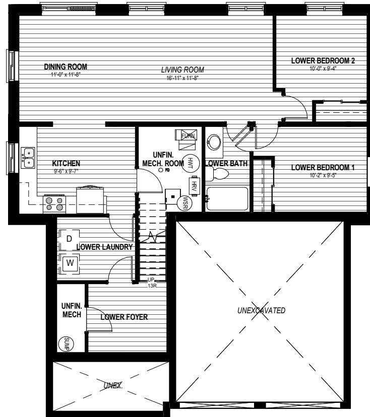
OPTIONAL FINISHED BASEMENT 1090 SQ.FT
