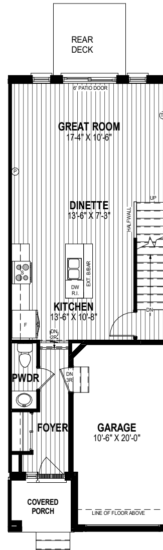
MAIN FLOOR PLAN 644 SQ.FT
