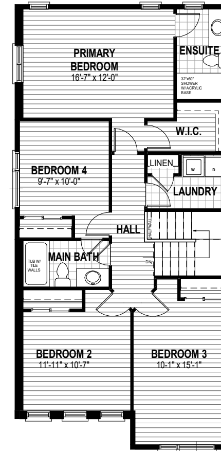
SECOND FLOOR PLAN ALT. 1 1073 SQ. FT.
