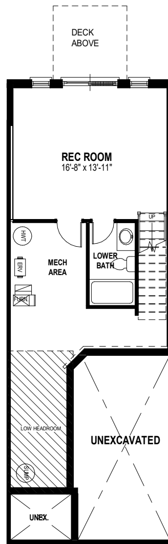
OPTIONAL FINISHED LOWER LEVEL PLAN 320 SQ. FT.
