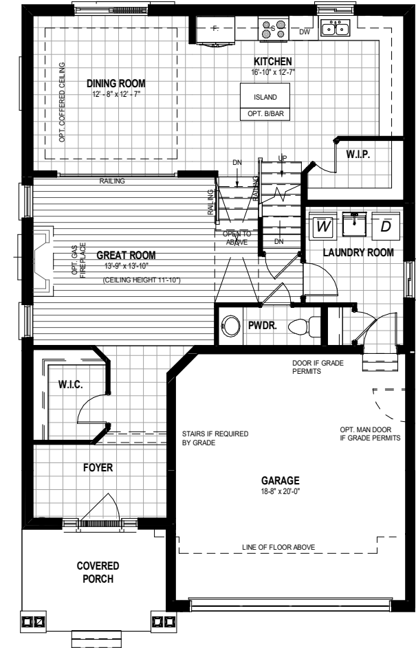
MAIN FLOOR PLAN ALT. KITCHEN LAYOUT 1068 SQ. FT.
