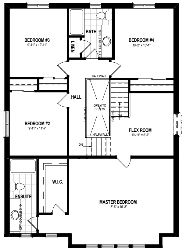
SECOND FLOOR PLAN 1375 SQ. FT.
