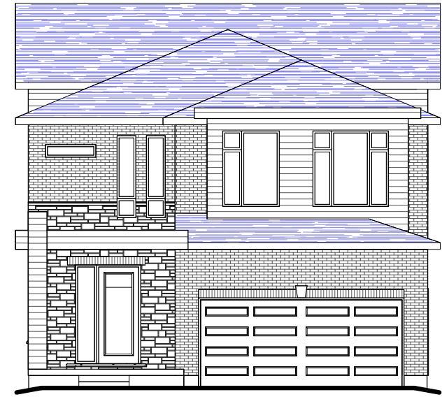
FRONT ELEVATION 'C'
