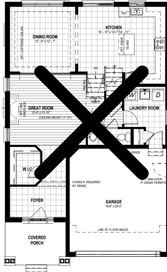
STANDARD MAIN FLOOR PLAN 1068 SQ. FT.
