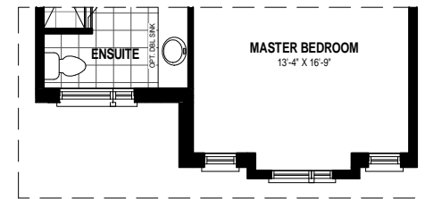
PARTIAL SECOND FLOOR PLAN ELV 'C' 1197 SQ.FT
