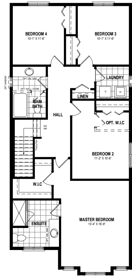
SECOND FLOOR PLAN ALT 1 1197 SQ.FT
