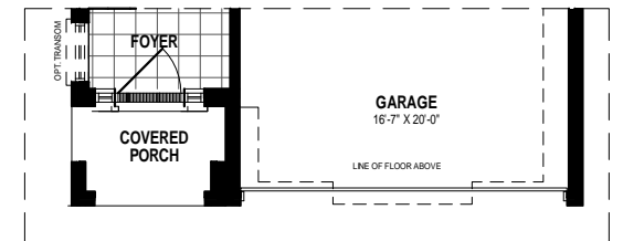
PARTIAL MAIN FLOOR ELV 'B' 897 SQ.FT
