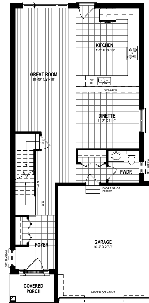
MAIN FLOOR PLAN ALT 2 897 SQ.FT
