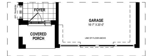
PARTIAL MAIN FLOOR ELV 'C' 897 SQ.FT
