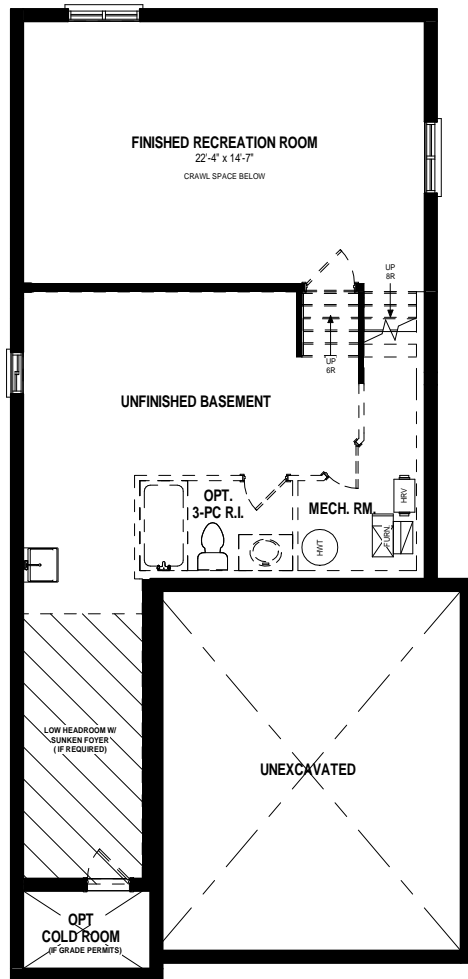
BASEMENT FLOOR PLAN 379 SQ.FT.
