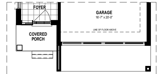
PARTIAL MAIN FLOOR PLAN ELEV "C" 923 SQ. FT.
