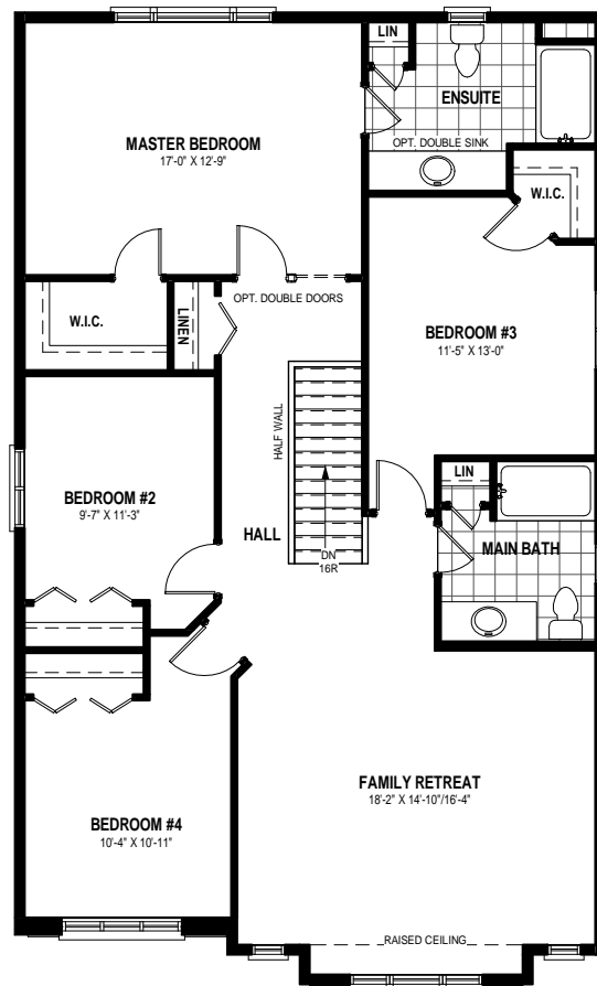
2ND FLOOR PLAN STANDARD ENSUITE 1,444 SQ.FT
