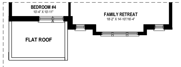
SECOND FLOOR PLAN ELEVATION 'C' 1416 SQ. FT.
