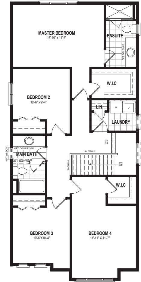
SECOND FLOOR PLAN ALT 2 1206 SQ. FT.
