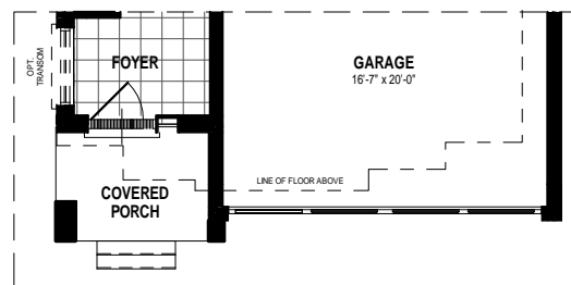
PARTIAL MAIN FLOOR PLAN ELV 'C' 901 SQ. FT.
