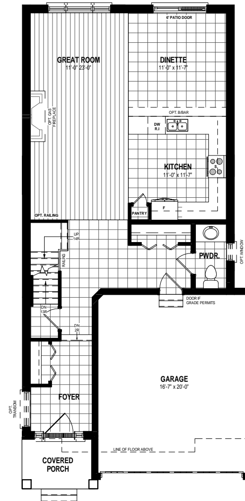
MAIN FLOOR PLAN. ALT 1 901 SQ. FT.
