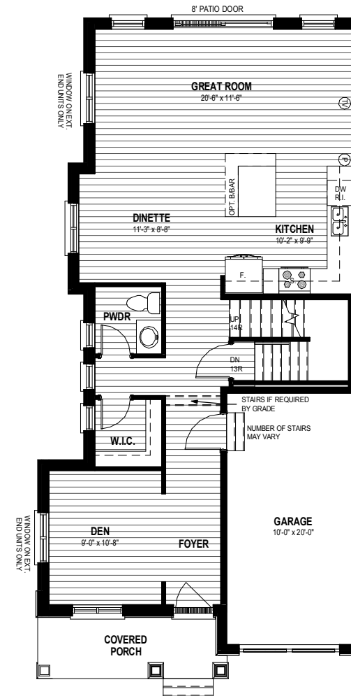
ALT. FLOOR PLAN EASY LIVING 920 SQ. FT.
