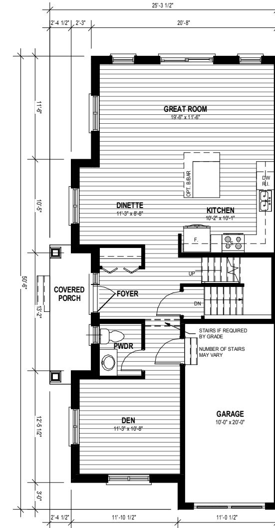
MAIN FLOOR PLAN 869 SQ. FT.
