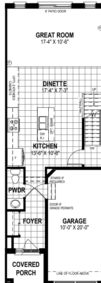
MAIN FLOOR PLAN 665 SQ.FT
