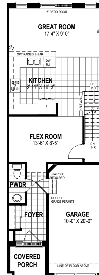
MAIN FLOOR PLAN ALT. 2 665 SQ.FT
