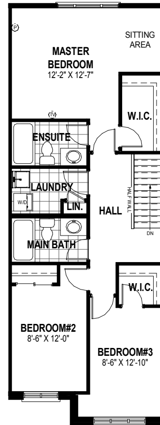
SECOND FLOOR PLAN ALT. 1 853 SQ.FT
