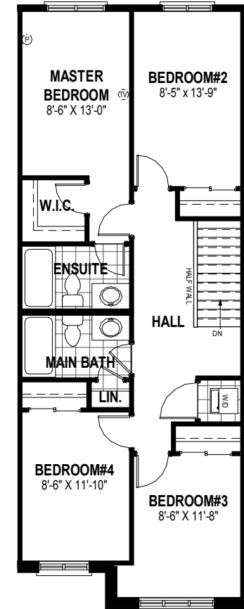
SECOND FLOOR PLAN ALT. 2 853 SQ.FT
