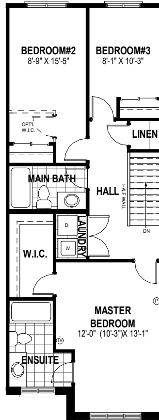
SECOND FLOOR PLAN 853 SQ.FT
