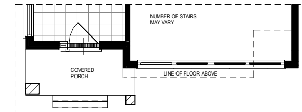
PARTIAL FIRST FLOOR PLAN ELV 'C' 1,116 SQ.FT
