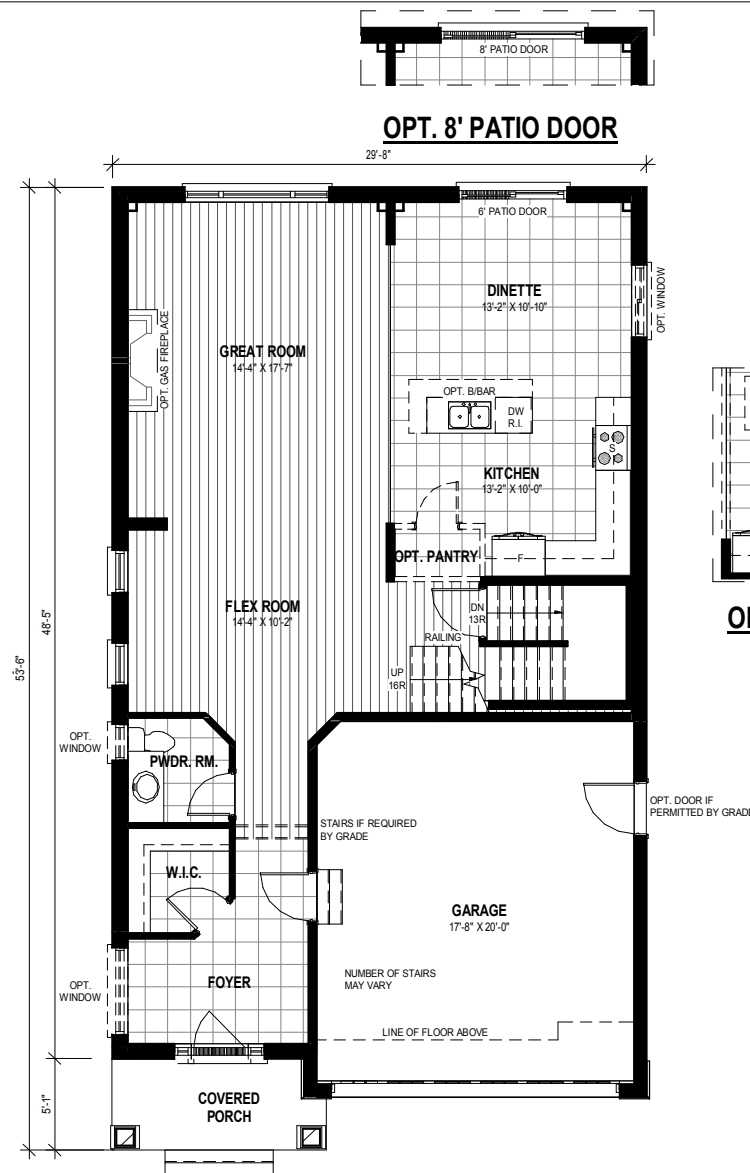
FIRST FLOOR PLAN ELV 'A' & 'B' 1,116 SQ.FT
