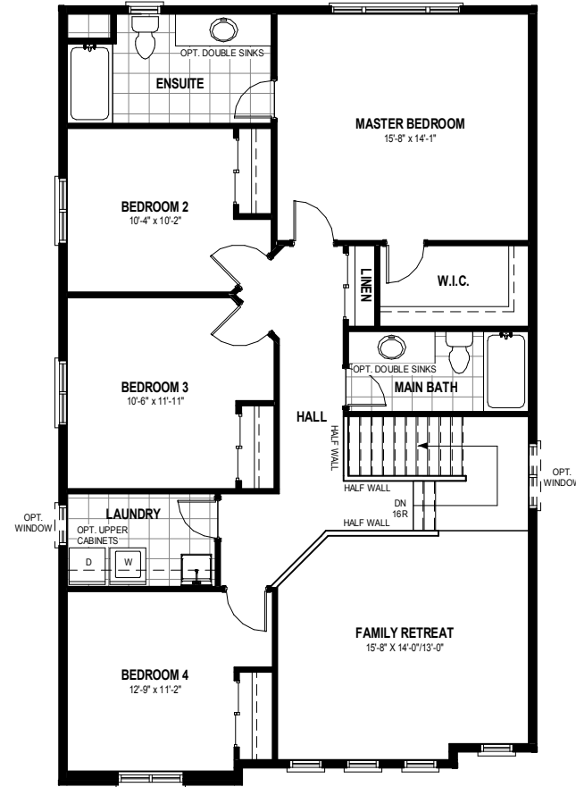
SECOND FLOOR PLAN ELV 'A' & 'B' 1,435 SQ.FT
