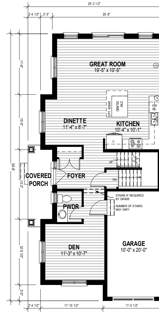
MAIN FLOOR PLAN 864 SQ. FT.
