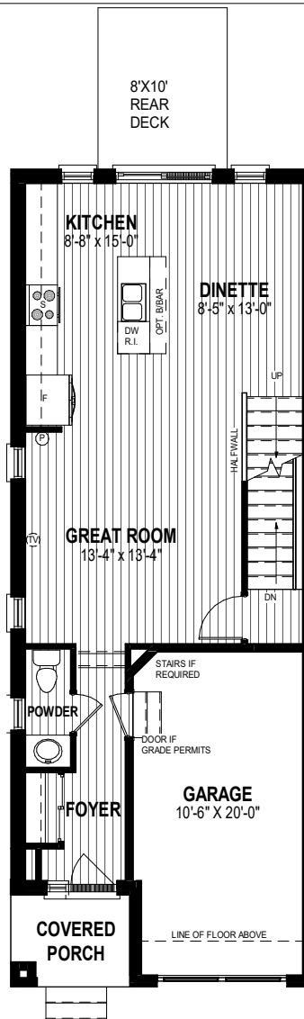
MAIN FLOOR PLAN ALT. 1 659 SQ.FT
