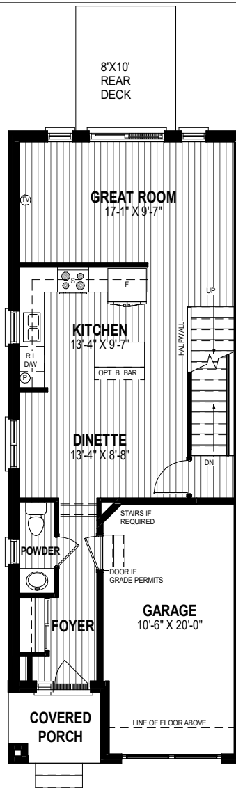
MAIN FLOOR PLAN ALT. 2 659 SQ.FT
