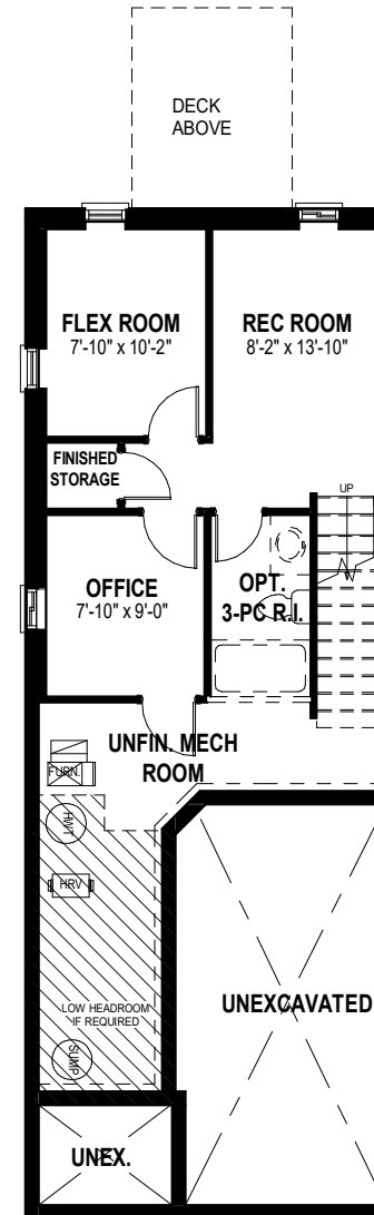
OPTIONAL FINISHED LOWER LEVEL ALT 2 411 SQ. FT.
