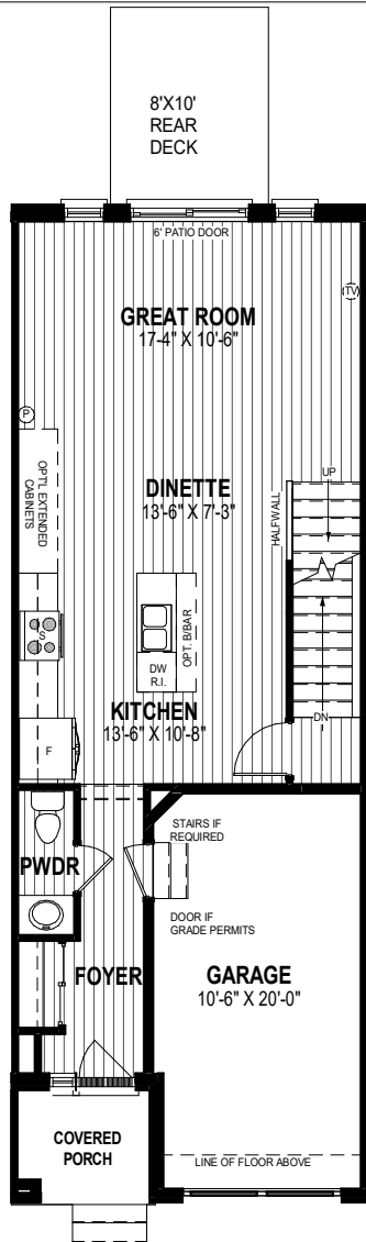
MAIN FLOOR PLAN 644 SQ.FT
