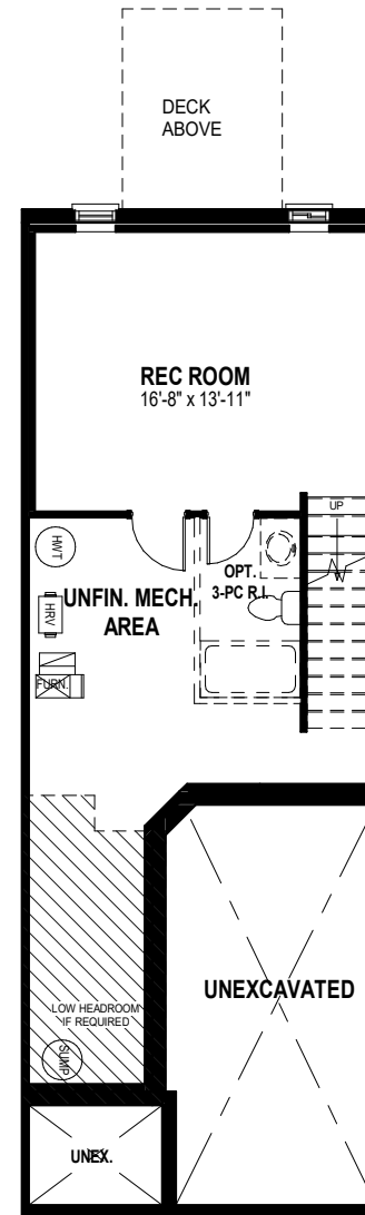
OPTIONAL FINISHED LOWER LEVEL PLAN 320 SQ. FT.
