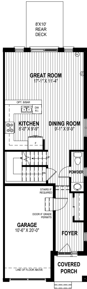
MAIN FLOOR PLAN ALT. 2 658 SQ.FT
