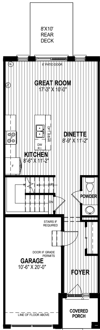
MAIN FLOOR PLAN 643 SQ.FT
