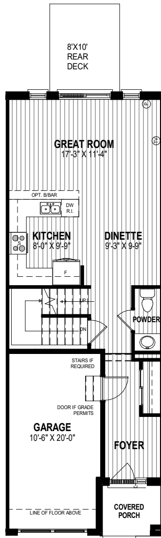
MAIN FLOOR PLAN ALT. 2 643 SQ.FT
