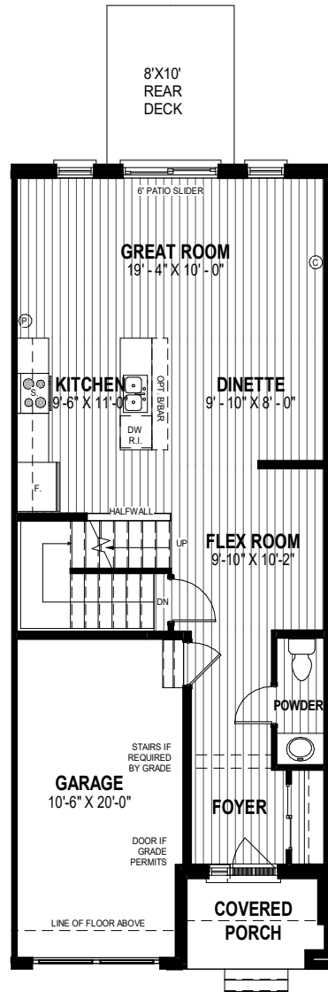
MAIN FLOOR PLAN 734 SQ. FT.
