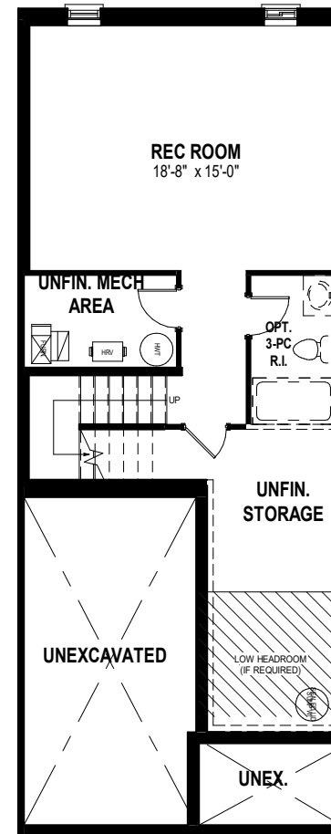
OPTIONAL FINISHED LOWER LEVEL FLOOR PLAN
