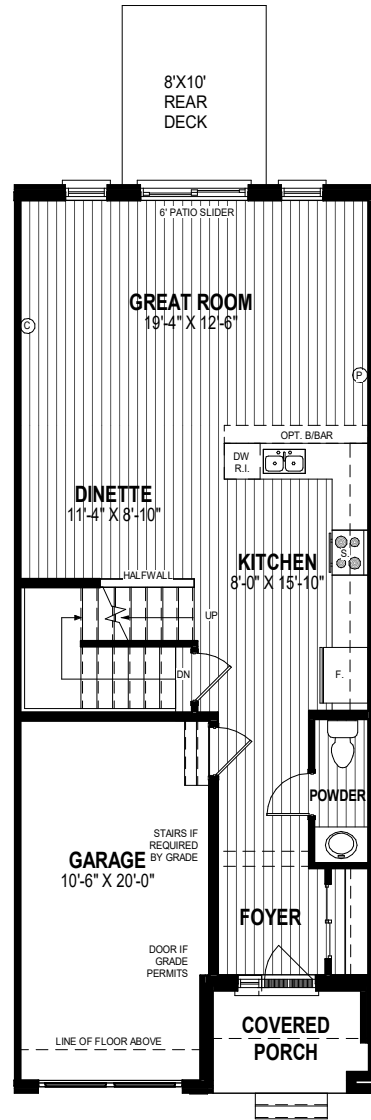
MAIN FLOOR PLAN ALT. 1 734 SQ. FT.
