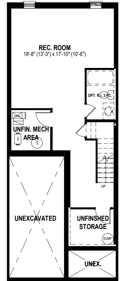
OPTIONAL FINISHED LOWER LEVEL FLOOR PLAN 582 SQ. FT.
