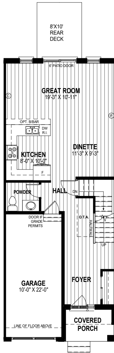
MAIN FLOOR PLAN ALT. 2 719 SQ.FT
