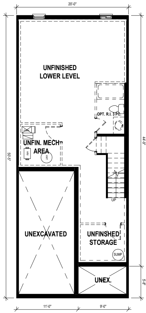
STANDARD UNFINISHED LOWER LEVEL FLOOR PLAN
