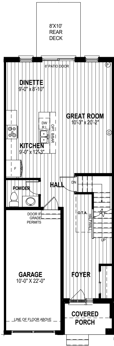
MAIN FLOOR PLAN 719 SQ.FT
