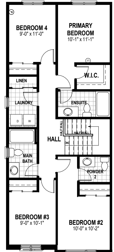
SECOND FLOOR PLAN ALT 2 968 SQ. FT.
