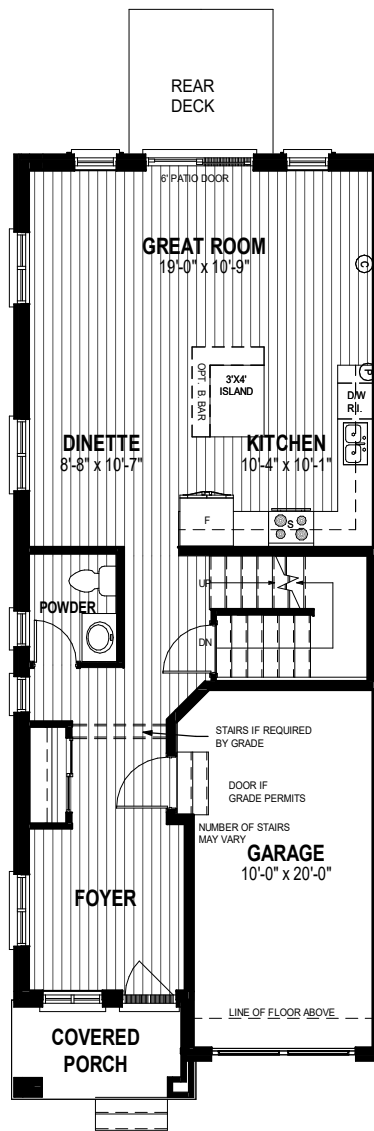
MAIN FLOOR PLAN ALT 1 778 SQ. FT.
