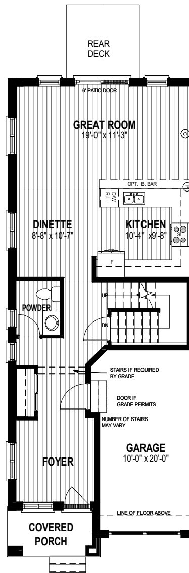
MAIN FLOOR PLAN ALT 2 778 SQ. FT.
