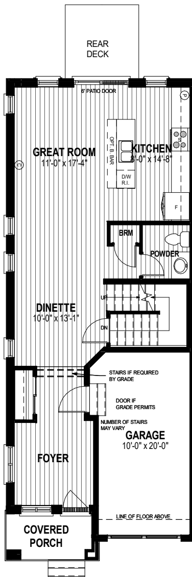
MAIN FLOOR PLAN 778 SQ. FT.
