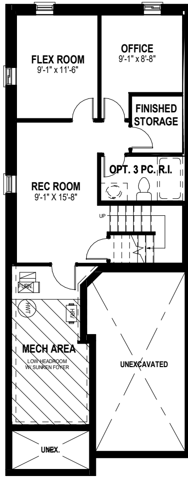
OPTIONAL FINISHED LOWER LEVEL ALT 2 550 SQ. FT.
