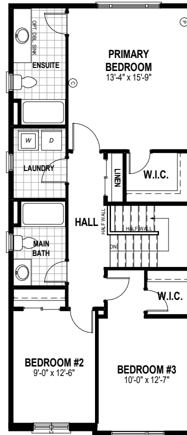
SECOND FLOOR PLAN 968 SQ. FT.
