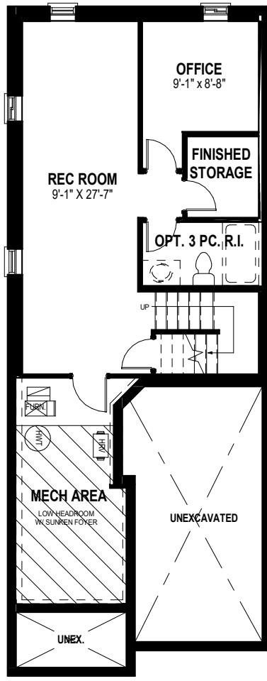
OPTIONAL FINISHED LOWER LEVEL ALT 1 550 SQ. FT.
