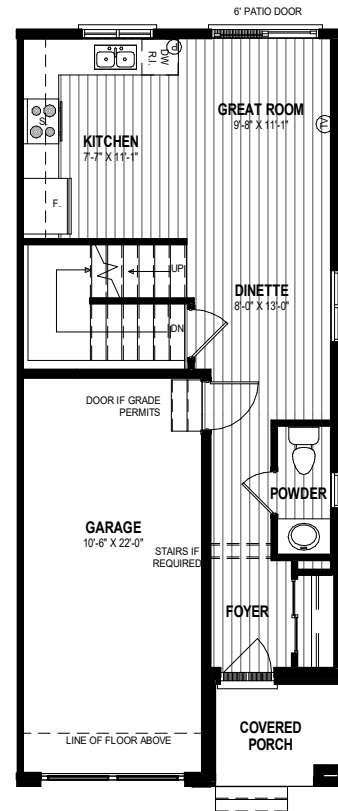
MAIN FLOOR PLAN ALTERNATE 491 SQ.FT
