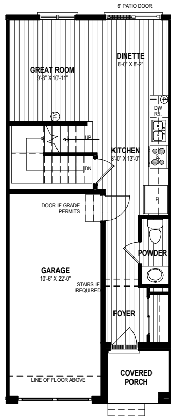
MAIN FLOOR PLAN 479 SQ.FT
