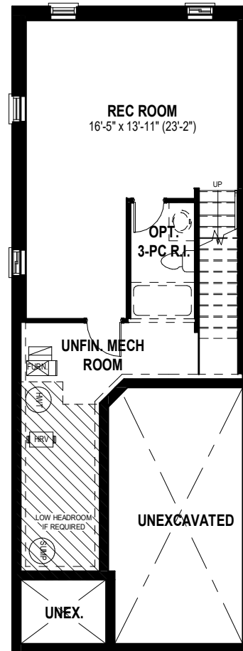
OPTIONAL FINISHED LOWER LEVEL ALT 1 411 SQ. FT.
