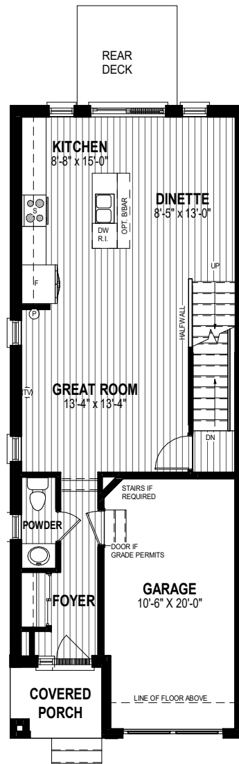
MAIN FLOOR PLAN ALT. 1 659 SQ.FT
