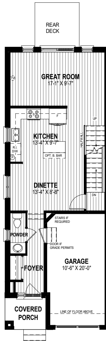
MAIN FLOOR PLAN ALT. 2 659 SQ.FT
