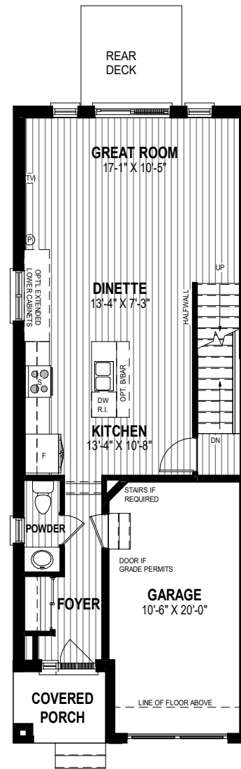
MAIN FLOOR PLAN 659 SQ.FT
