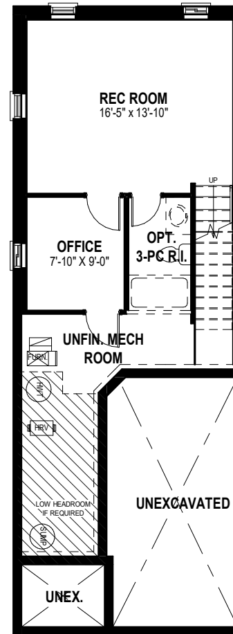
OPTIONAL FINISHED LOWER LEVEL ALT 2 411 SQ. FT.
