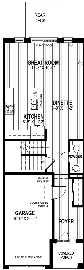
MAIN FLOOR PLAN ALT. 1 643 SQ.FT
