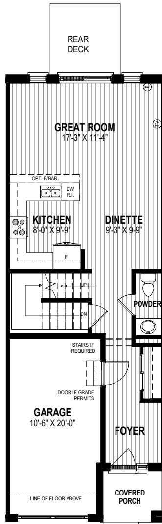
MAIN FLOOR PLAN ALT. 2 643 SQ.FT
