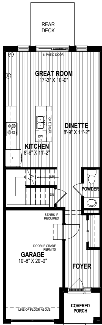
MAIN FLOOR PLAN 643 SQ.FT
