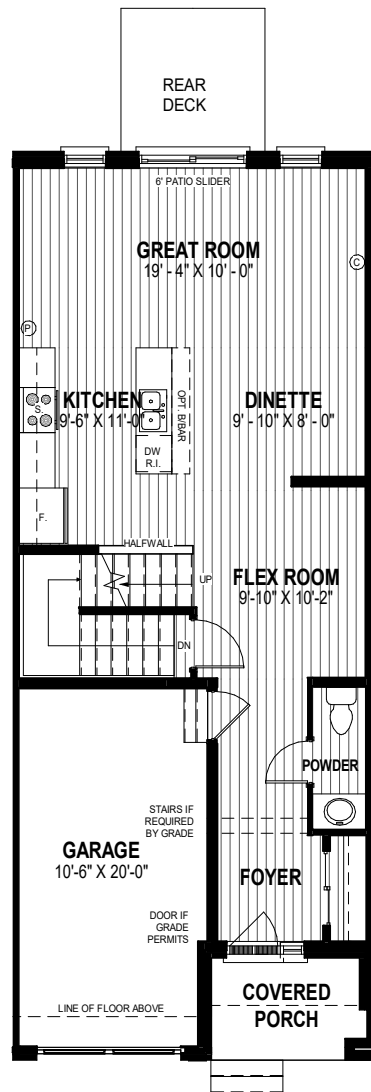
MAIN FLOOR PLAN 734 SQ. FT.
