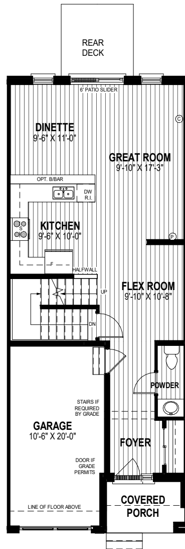
MAIN FLOOR PLAN ALT. 2 734 SQ. FT.
