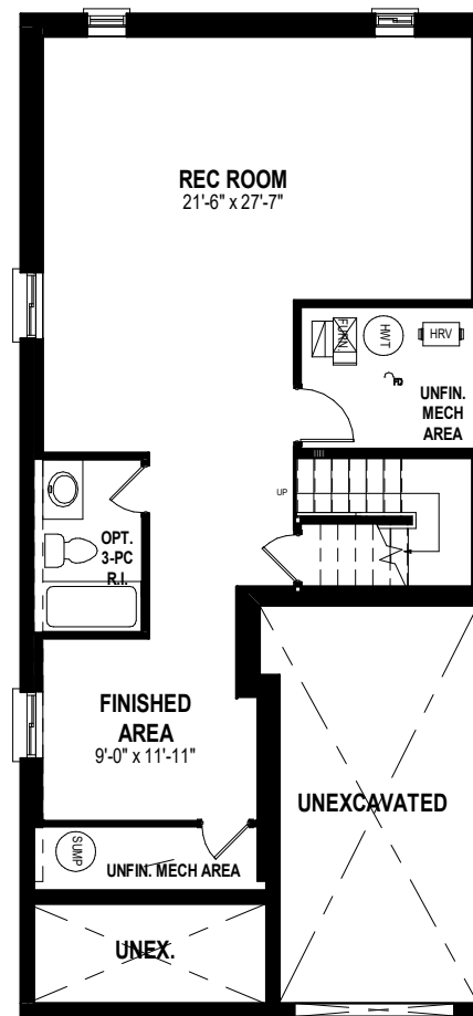
OPTIONAL FINISHED LOWER LEVEL FLOOR PLAN 764 SQ. FT.
