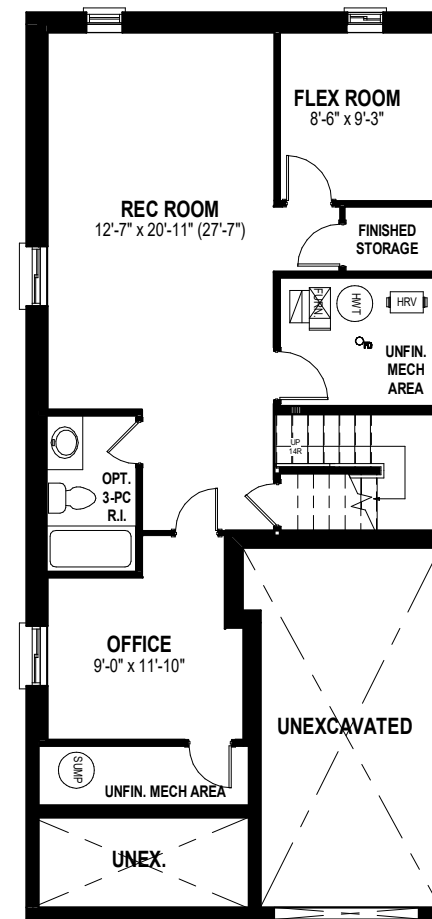
OPTIONAL FINISHED ALT 2 LOWER LEVEL FLOOR PLAN 764 SQ. FT.
