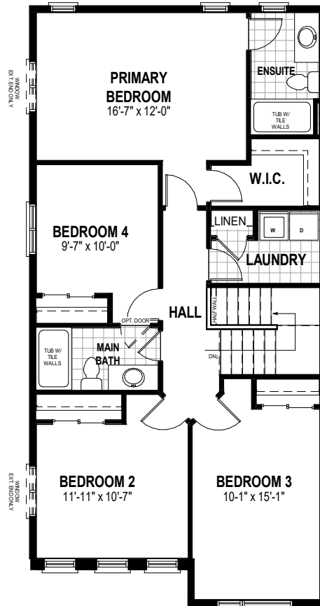
SECOND FLOOR PLAN ALT. 1 1073 SQ. FT.
