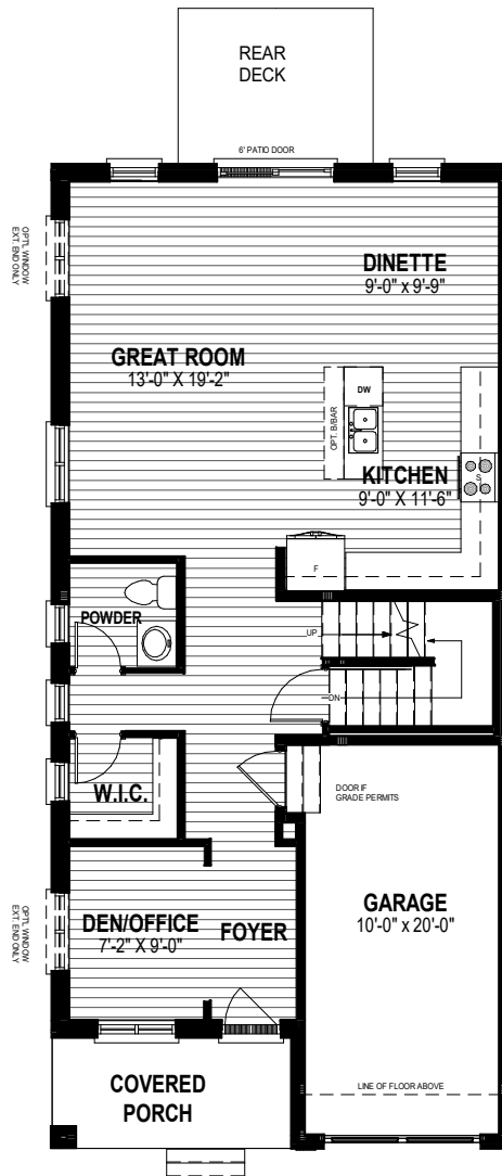
MAIN FLOOR PLAN 902 SQ. FT.
