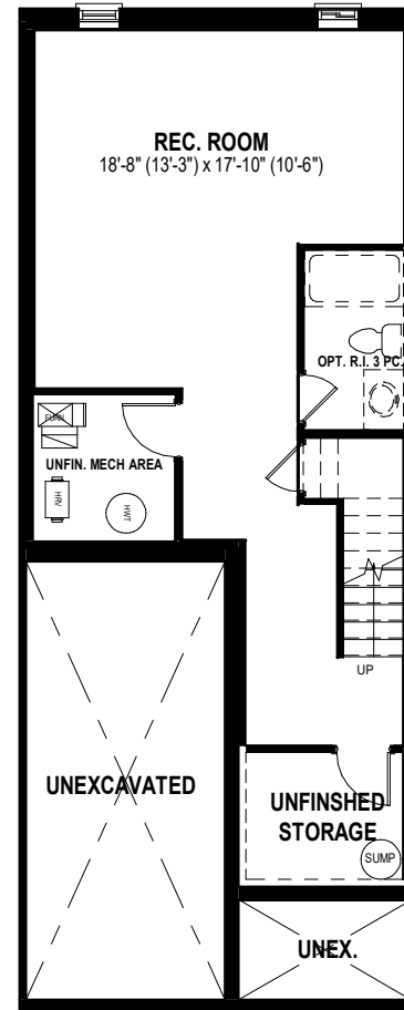
OPTIONAL FINISHED LOWER LEVEL FLOOR PLAN 582 SQ. FT.
