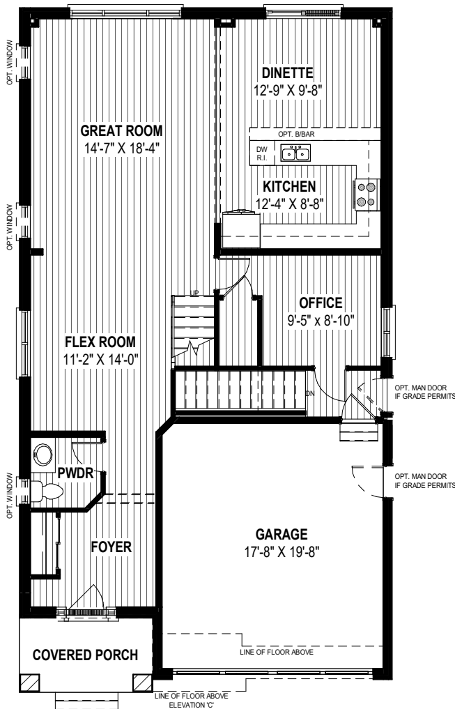
MAIN FLOOR PLAN ALT 1 1,155 SQ.FT
