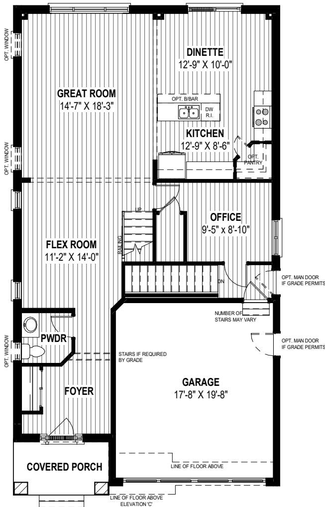
MAIN FLOOR PLAN 1,155 SQ.FT
