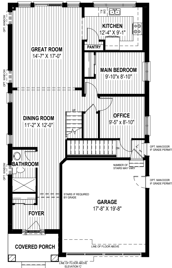
MAIN FLOOR PLAN ALT 2 1,155 SQ.FT
