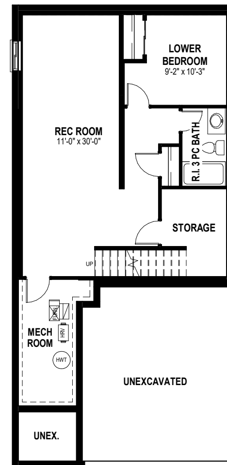
OPTIONAL FINISHED LOWER LEVEL FLOOR PLAN 739 SF
