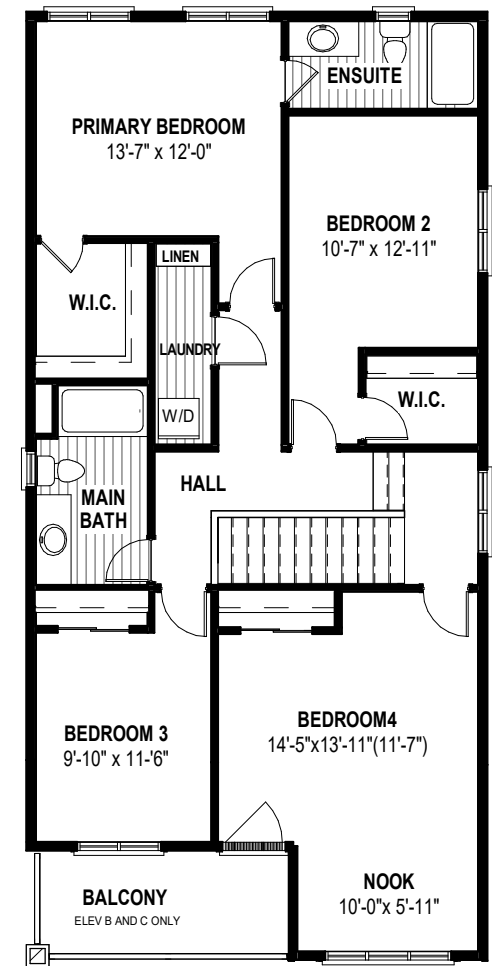
SECOND FLOOR PLAN ALT 1 1267 SQ.FT ELEV B SHOWN
