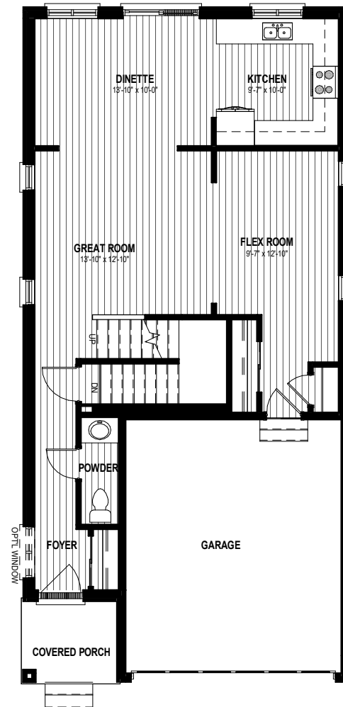
MAIN FLOOR PLAN ALT. 1 945 SQ.FT
