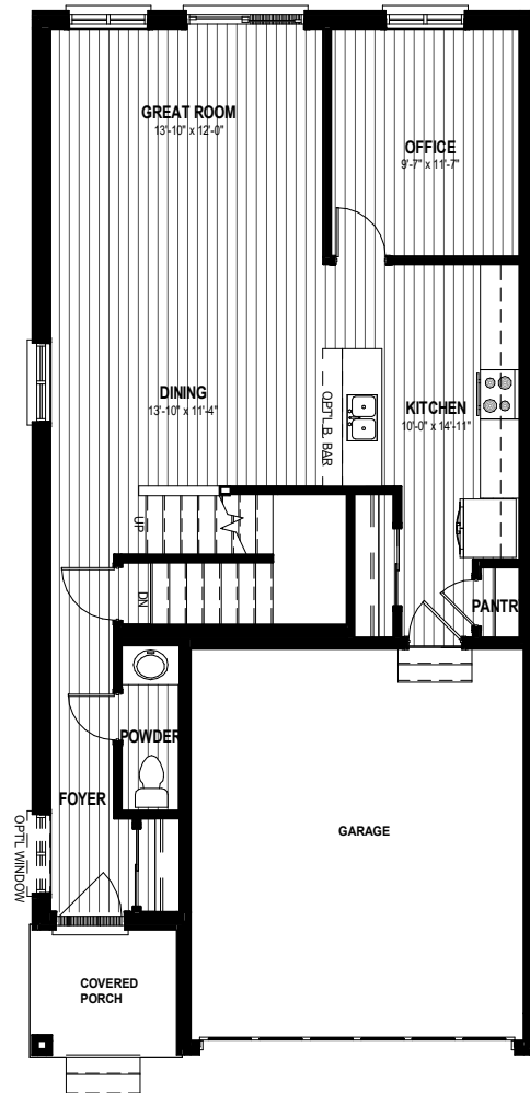
MAIN FLOOR PLAN 945 SQ.FT
