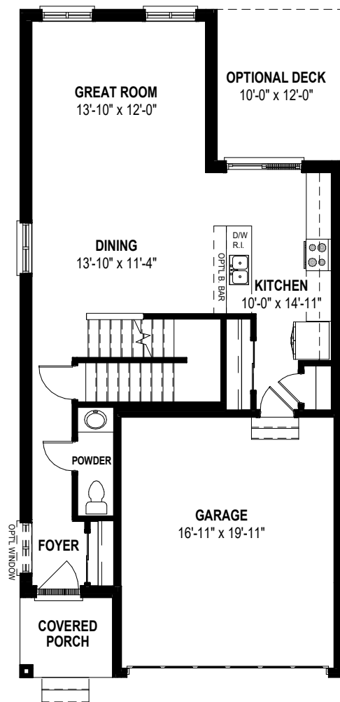
MAIN FLOOR PLAN 825 SQ.FT
