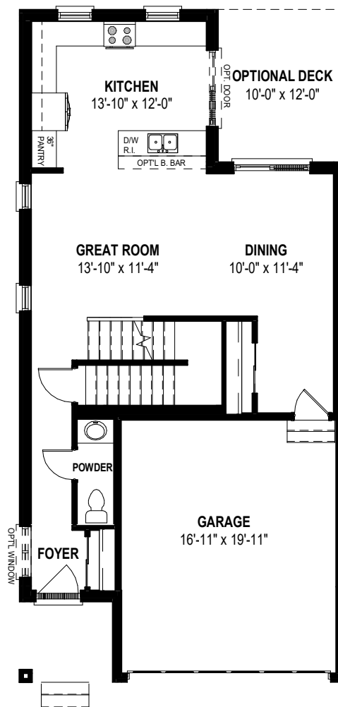
MAIN FLOOR PLAN ALT. 1 825 SQ.FT
