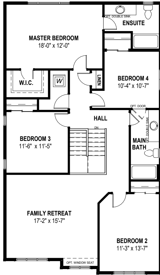
SECOND FLOOR PLAN 1,509 SQ.FT
