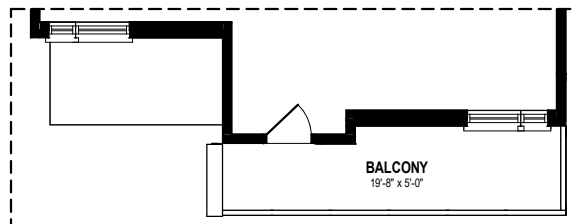
SECOND FLOOR ALT. PLAN ELEVATION 'C' 1571 SQ. FT.
