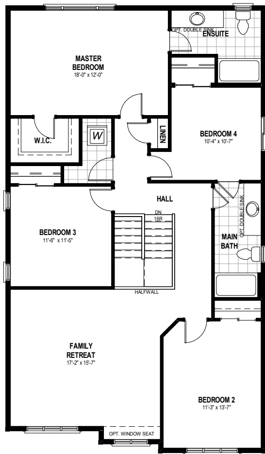
SECOND FLOOR PLAN 1,509 SQ.FT
