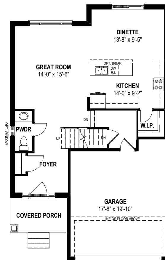
MAIN FLOOR PLAN 858 SQ.FT
