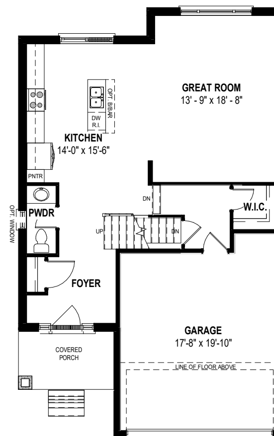
MAIN FLOOR PLAN ALT 2 858 SQ.FT
