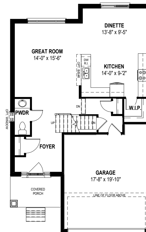
MAIN FLOOR PLAN ALT 1 858 SQ.FT
