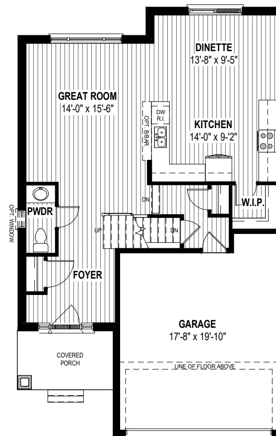
MAIN FLOOR PLAN ALT 1 858 SQ.FT
